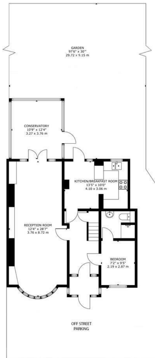
GROUND FLOOR
